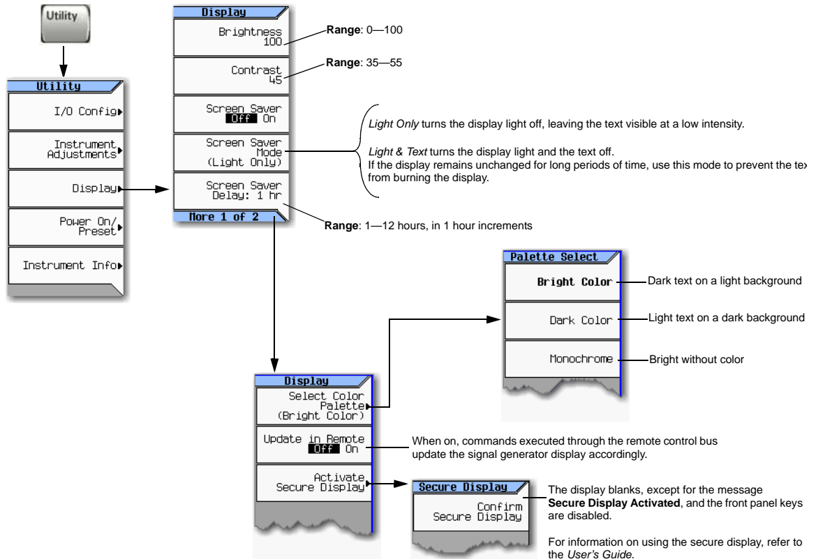
Figure 2-3 Display Softkeys
